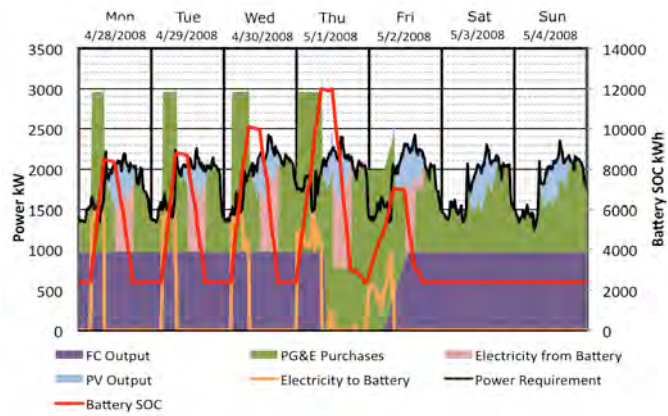
Fig. 4 Optimized May 2008 Week NaS Battery Operation Notice that the battery is left discharged over the weekend. Round-trip losses are significant for NaS batteries, and 30% is the average here. In general, the battery is charged in the early morning hours and discharged during the following afternoon. Strangely the state-of-charge is considerably lower during a fuel cell outage, a surprising result driven by the off peak demand charges.
